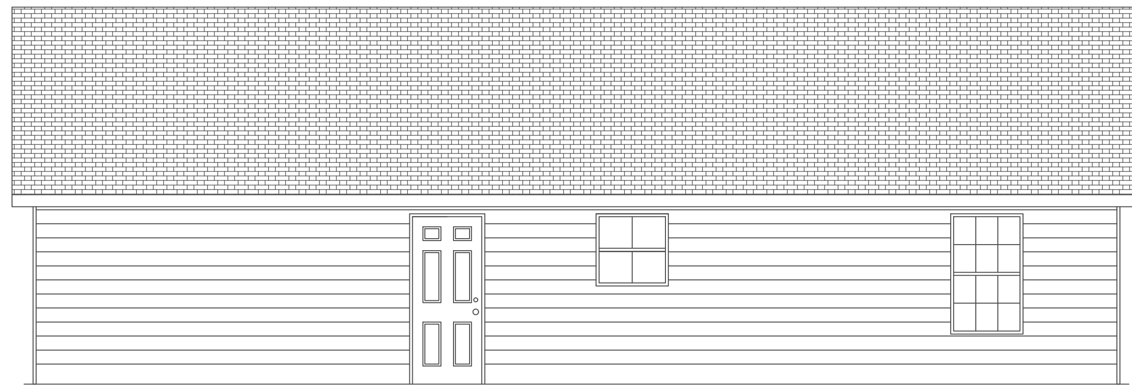
REAR ELEVATION 1/4" = 1'0"
