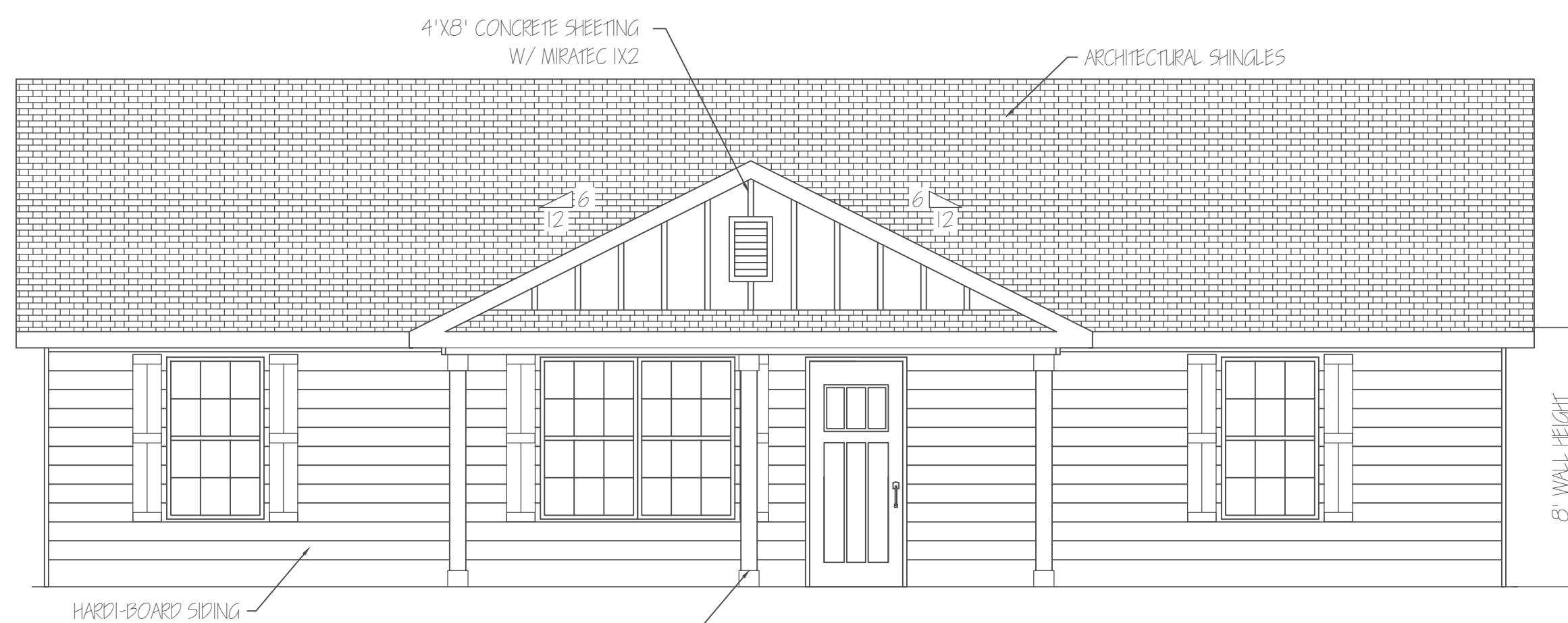
FRONT ELEVATION 1/4" = 1'0"
