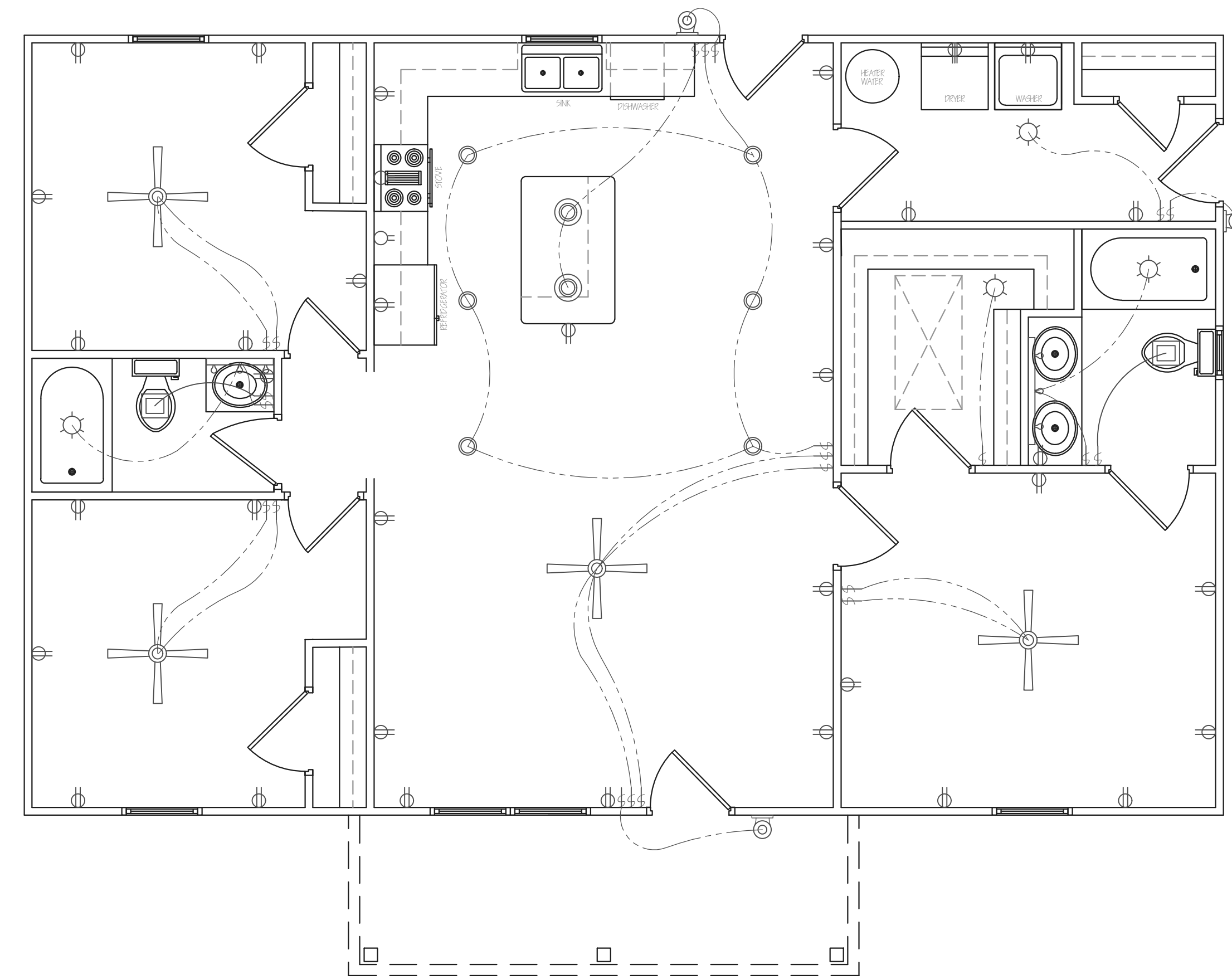
ELECTRICAL PLAN 1/4" = 1'0"
