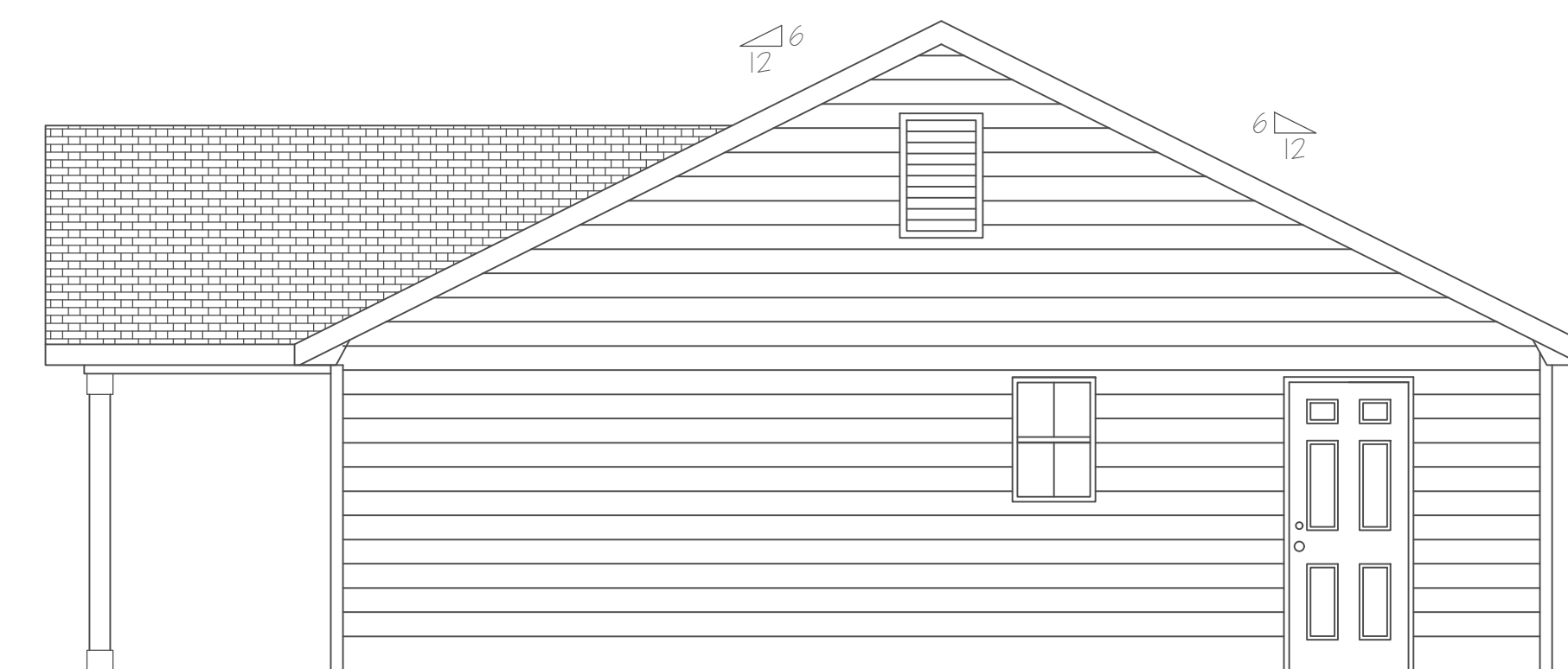
RIGHT ELEVATION 1/4" = 1'0"
